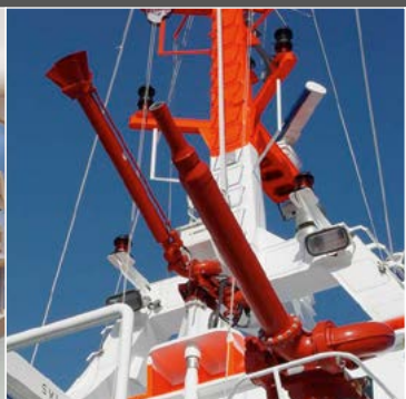
Slew drive for fire-gun
